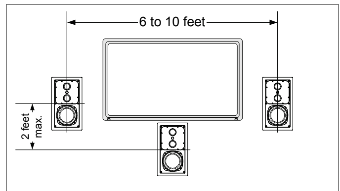
Height measured to center of speaker from floor
