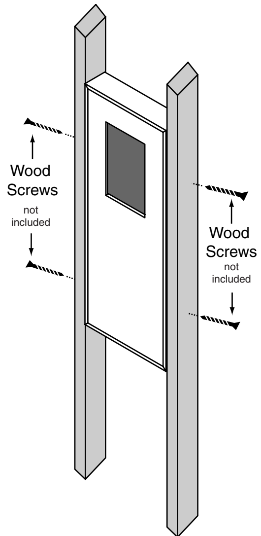
Rectangle back box shown as an example
