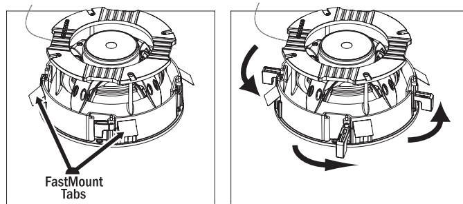
Figure 4: Original Series Medium Round Speaker Installation
