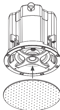
FIGURE 15: GRILLE INSTALLATION
