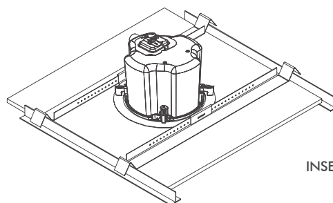
FIGURE 16: SCREW C-BRACKET TO TILE SUPPORT RAILS
