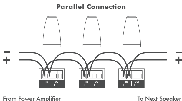
FIGURE 17: PARALLEL CONNECTION
