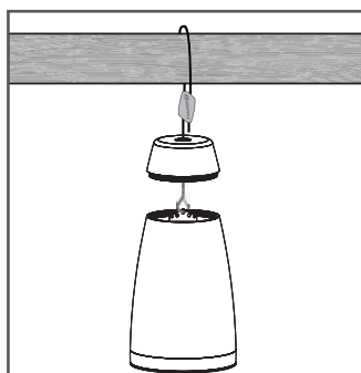
FIGURE 7: MAIN SUPPORT
