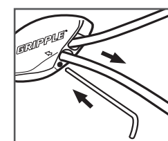
FIGURE 11: RELEASE CABLE
